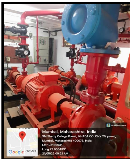
Collection system from borewell and BMC
